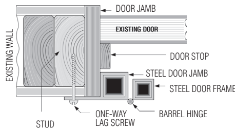
INSET MOUNT W/SURFACE TABS
