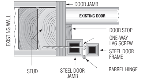
INSET MOUNT
