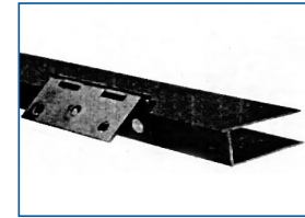
Extruded aluminum hinge side adjustment channel
