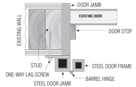
SURFACE MOUNT W/TABS
