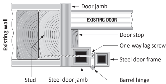
Inset mount
